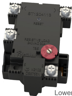
11122: Thermostat Robert Shaw ST204113 red dial
