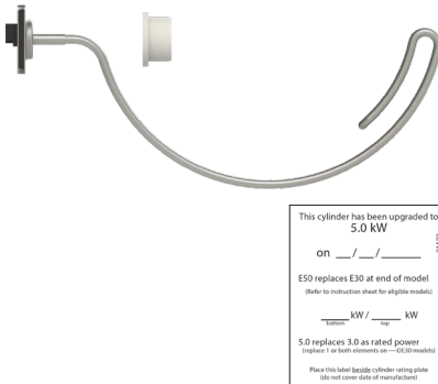
21253: Element 5kW Ø590-685
