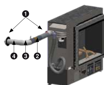
1. Direct flue kit - ASPDFK 2. Flue transition - LSFEXTKIT01 3. 45° bends - ESBEND 4. Flue pipe - ESPIPE900
