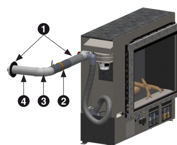
1. Direct flue kit - ASPDFK 2. Flue transition - LSFEXKIT01 3. 45° bends - ESBEND 4. Flue pipe - ESPIPE900
