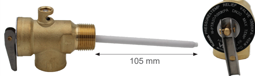
20573: TPR valve 1000 kPa, 46 kW, 99 °C, DN20 Male inlet, female outlet.
