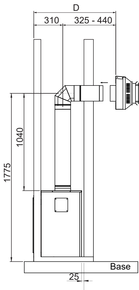
RDV3611 Short Horiz. Flue Kit A (R3660)
