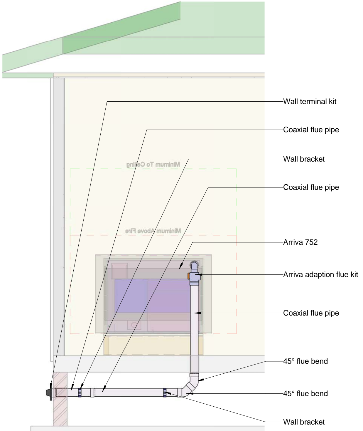
Section Along - Rear View
