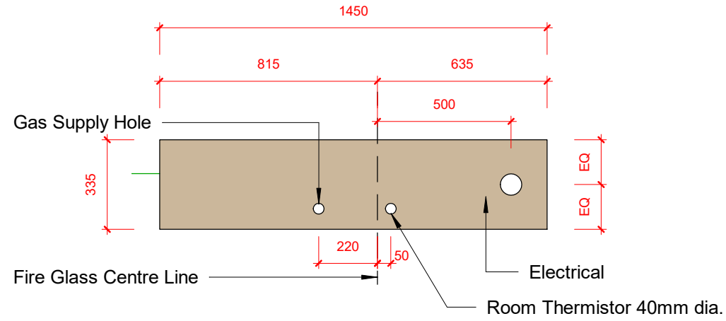
Fire Platform - Plan View 1 : 20
