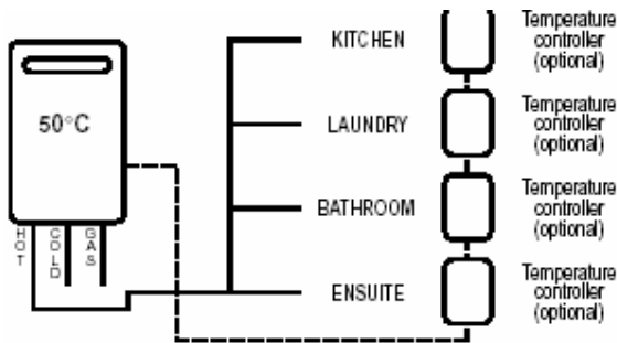
Diagram 1 - 50°C Appliance
