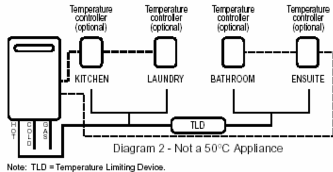
Diagram 2 - Not a 50°C Appliance
