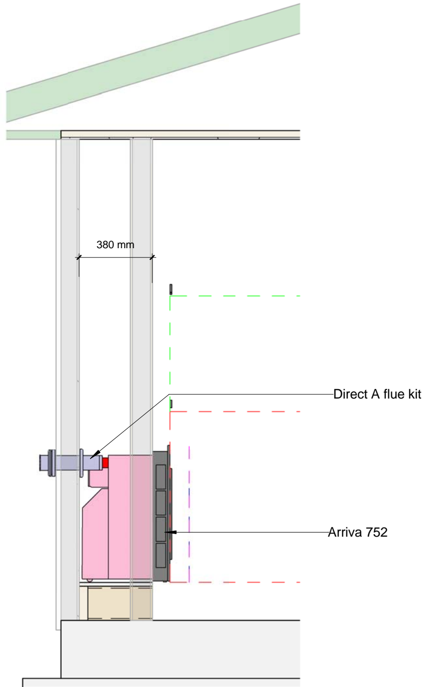
Section Across
