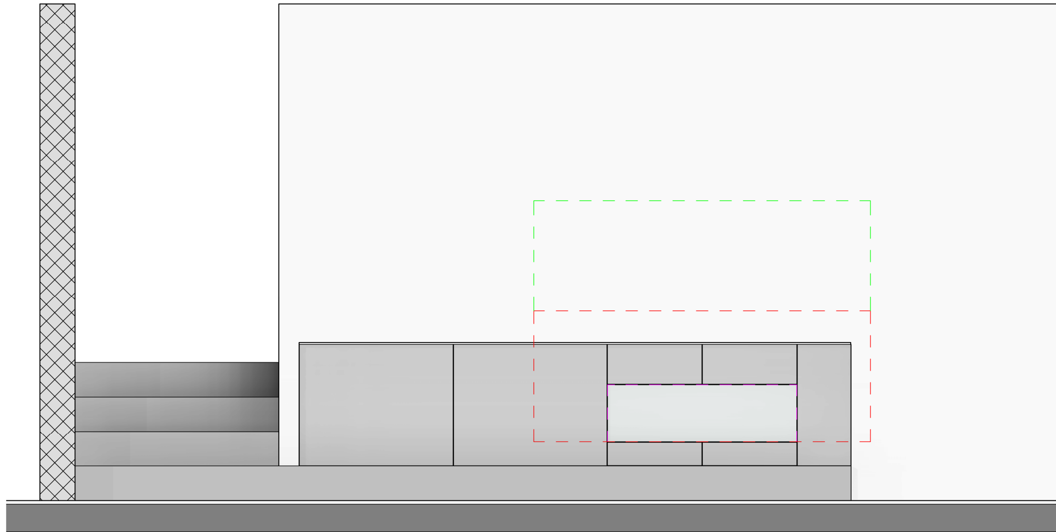
Elevation Front 1 : 20
