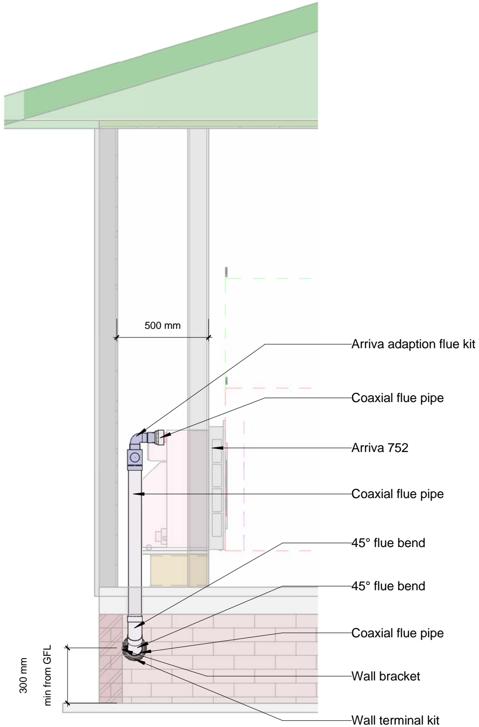
Section Across
